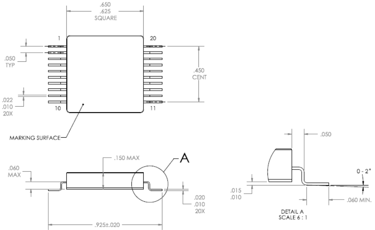
FIGURE 2 Model 1420 Package Outline
